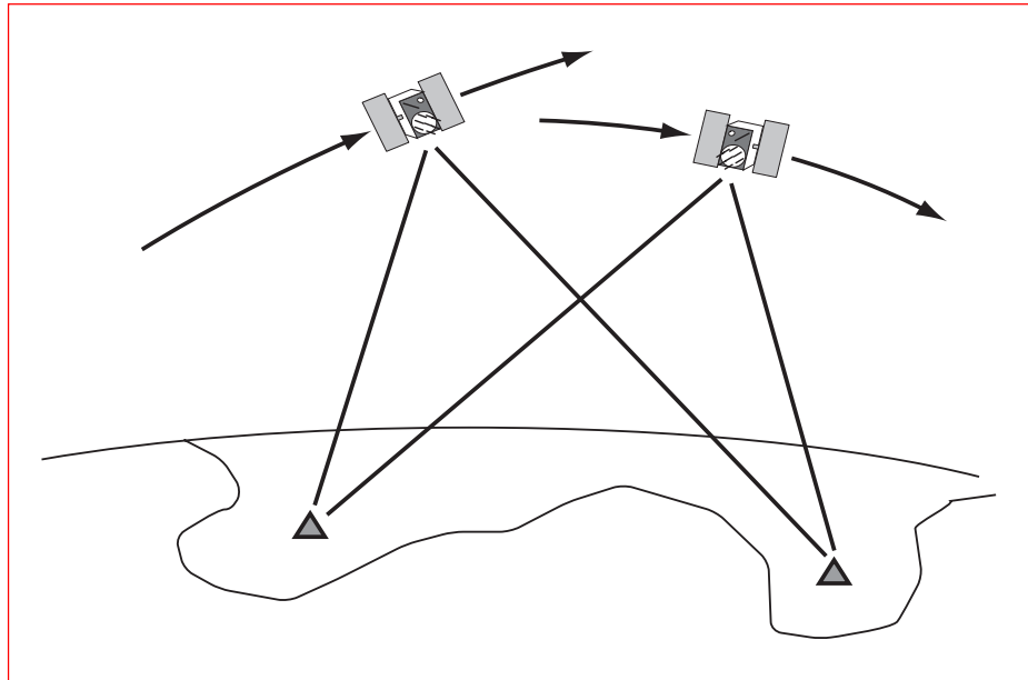
Double Differencing
