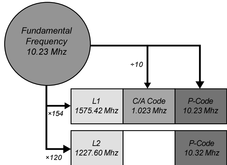
GPS Signal Structure
