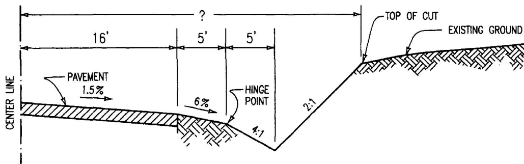
TYPICAL CROSS-SECTION
