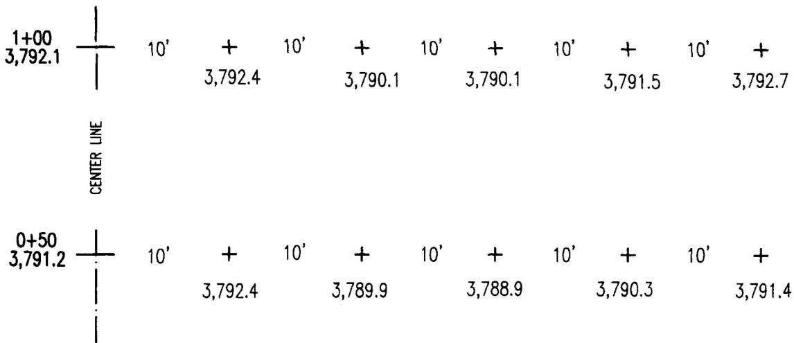
CROSS-SECTIONS OF EXISTING GROUND
